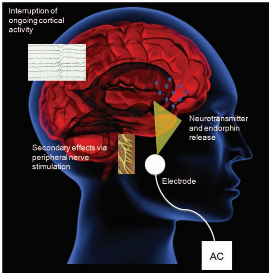
Figure 6. Putative mechanisms of action of alternating current (AC) stimulation. Some potential mechanisms of AC stimulation are 1) release or neurotransmitters, 2) interruption of ongoing cortical activity, and 3) secondary effects via peripheral nerve stimulation.
