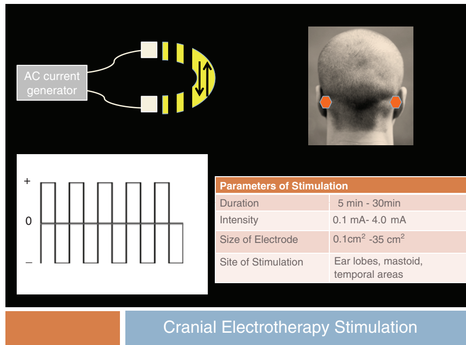
Figure 4. Main characteristics of cranial electrotherapy stimulation (CES). The orange polygons represent AC electrodes (usually placed on mastoid process or ear lobes). The graph represents electrical current polarity changes over time.
