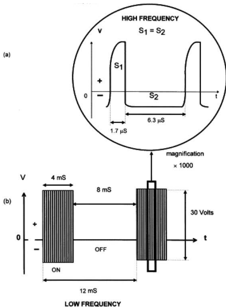
Figure 5. Main characteristics of Limoge and Lebedev current stimulation. a, Wave trains are composed of successive impulse waves of a particular shape: one positive impulse (S1) of high intensity and short duration, followed by a negative impulse (S2) of weak intensity and long duration. The high-frequency current is regularly interrupted by a low-frequency cycle (4 mS “ON” + 8 mS “OFF”). b, Headset positioning of electrodes in Limoge and Lebedev current stimulation (adapted with permission from Limoge and others 1999).
