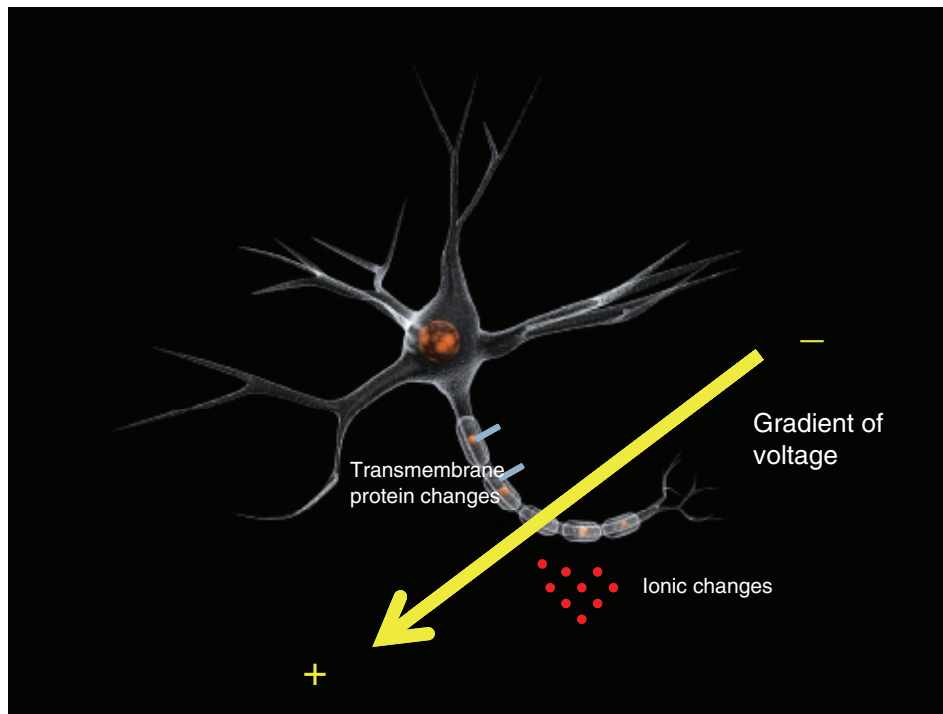
Figure 2. Putative mechanisms of action of transcranial direct current stimulation. The constant gradient of voltage induces ionic shifts and transmembrane protein changes that result in changes to cortical excitability.
